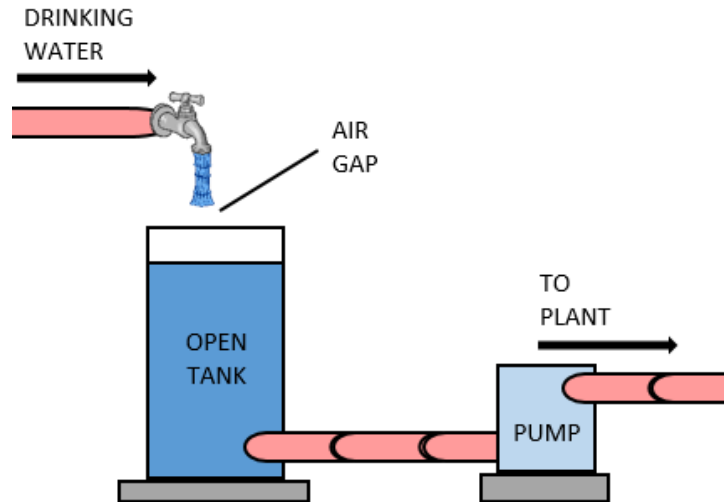
Figure 7.16: A backflow prevention diagram 72
