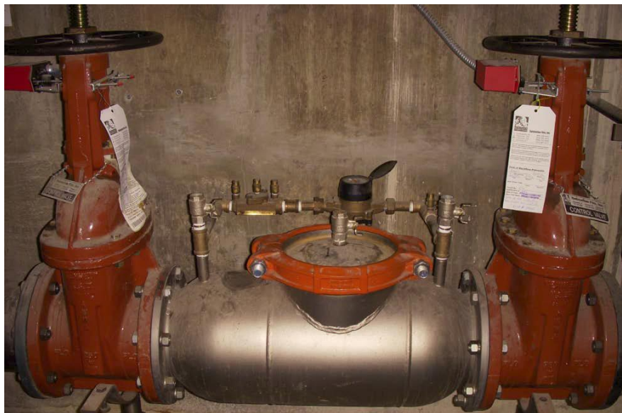
Figure 7.21: A backflow prevention device 77
