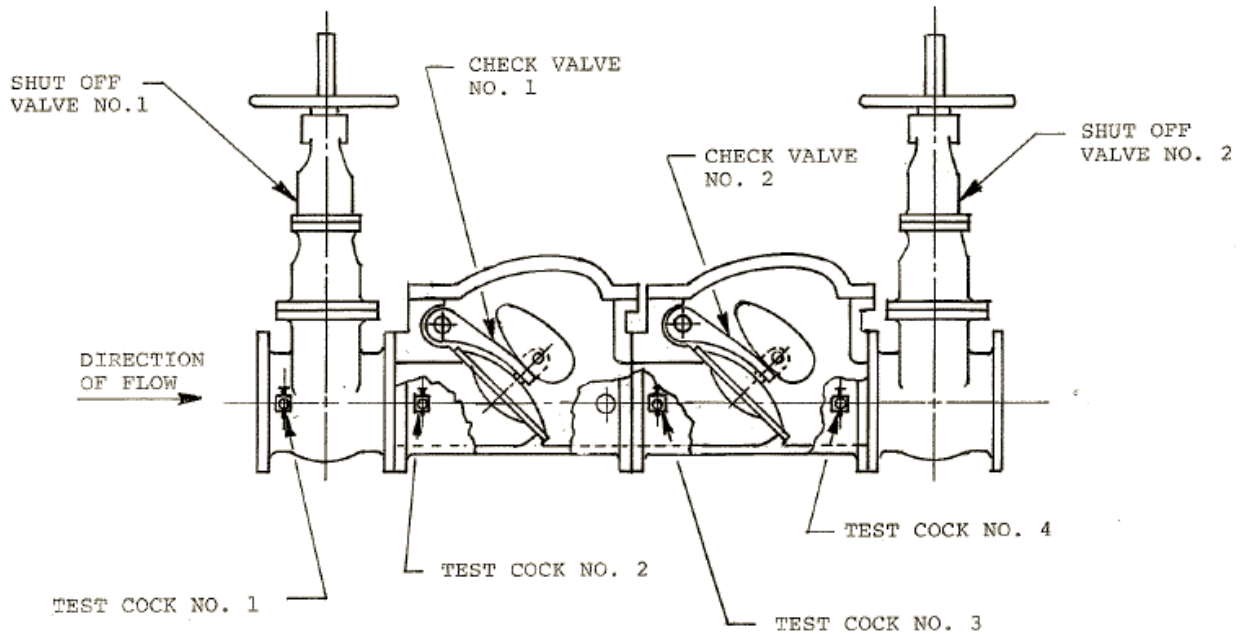
Figure 7.20: A backflow prevention device diagram 76
