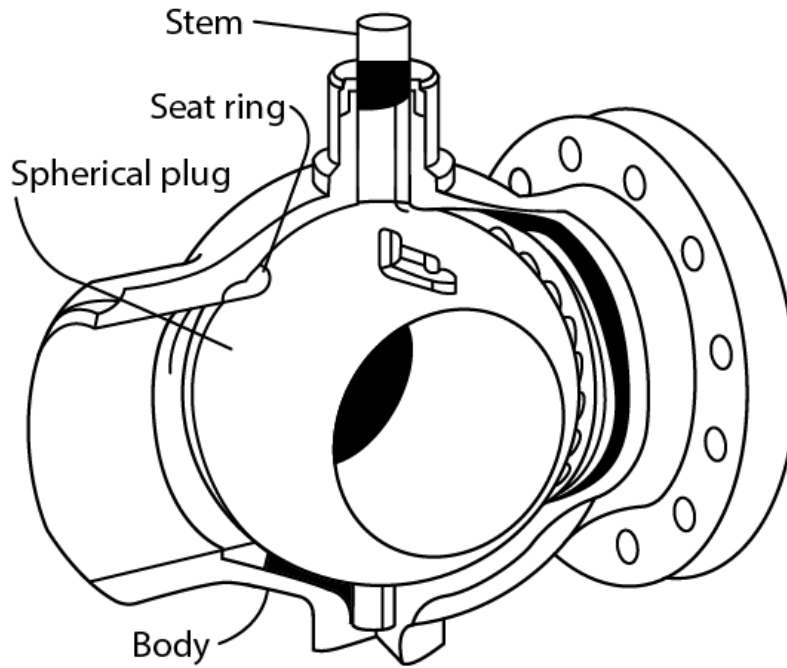
7.12: Ball Valve 68
