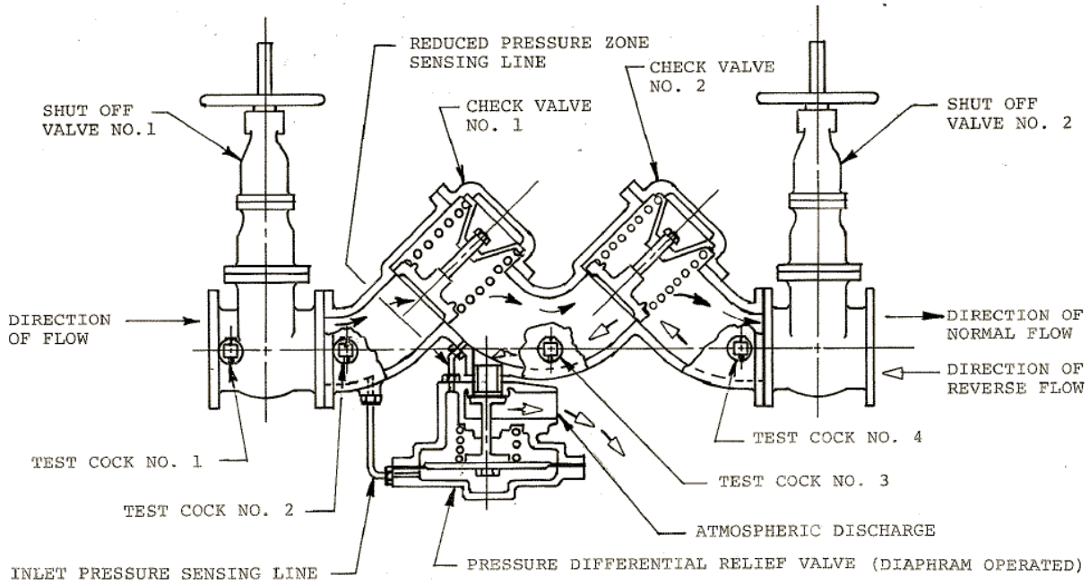
Figure 7.18: A double check valve diagram 74
