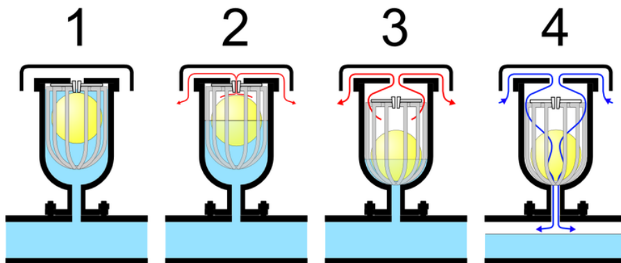
Figure 4.5: Air valve model 31
