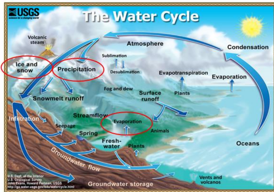
Figure 2.2: The hydrologic cycle 11
