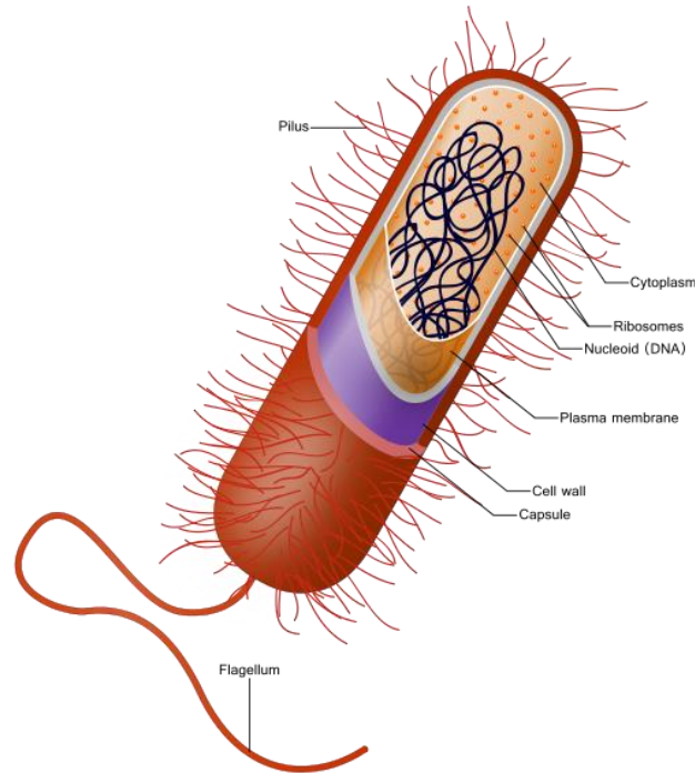
Figure 3.1: Prokaryote cell 18
