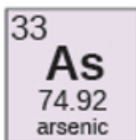
Figure 3.3: Arsenic on the periodic table 20
