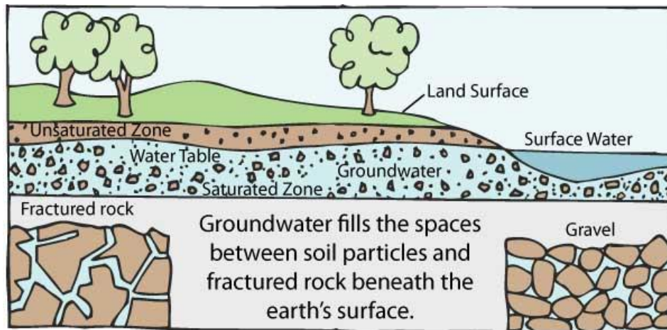
Figure 2.3: Groundwater movement 12
