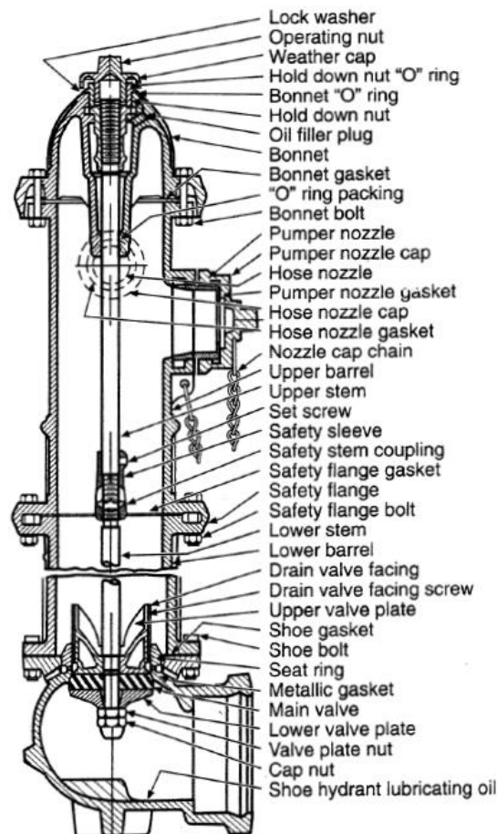
Figure 8.10: A dry barrel fire hydrant diagram 87
