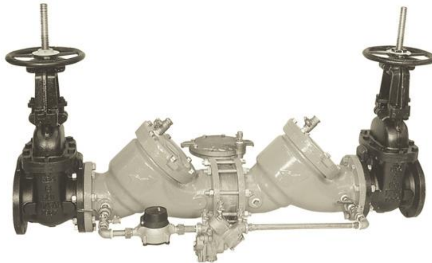
Figure 7.19: A double check valve 75
