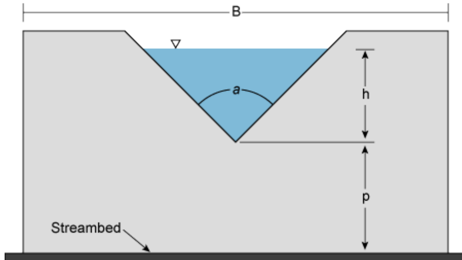
Figure 9.3: A triangular or V notch weir diagram 91
