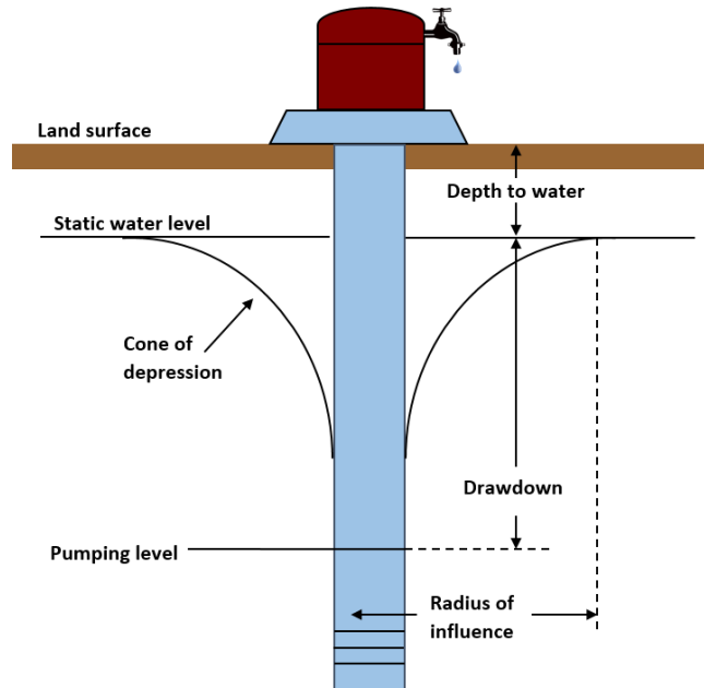
Figure 11.5: This diagram demonstrates how groundwater is measured through static and pumping levels 105
