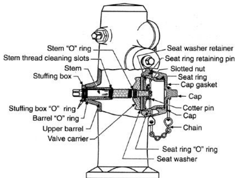
Figure 8.11: A wet barrel fire hydrant diagram 88
