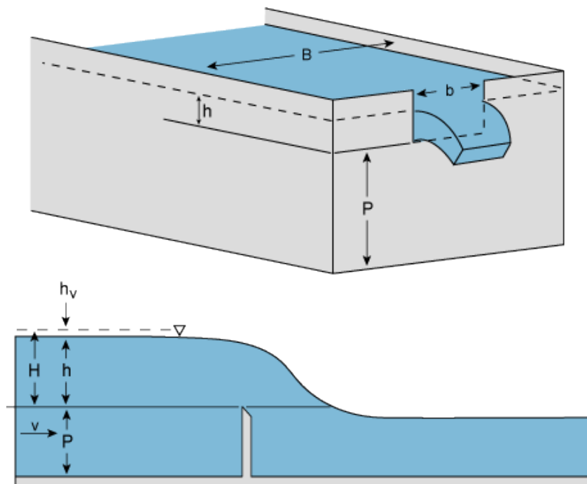
Figure 9.4: A rectangular thin plate weir diagram 92
