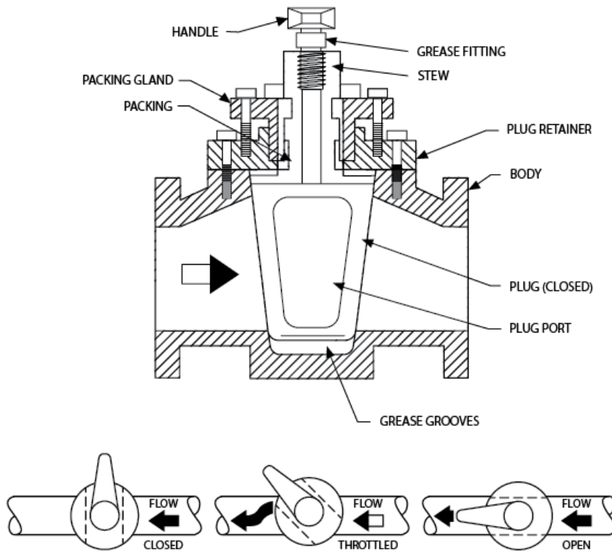
7.10: Plug Valve 66
