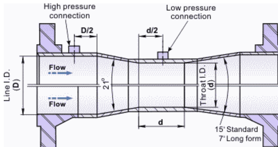
Figure 9.1: A Schematic diagram of venturi meter 89
