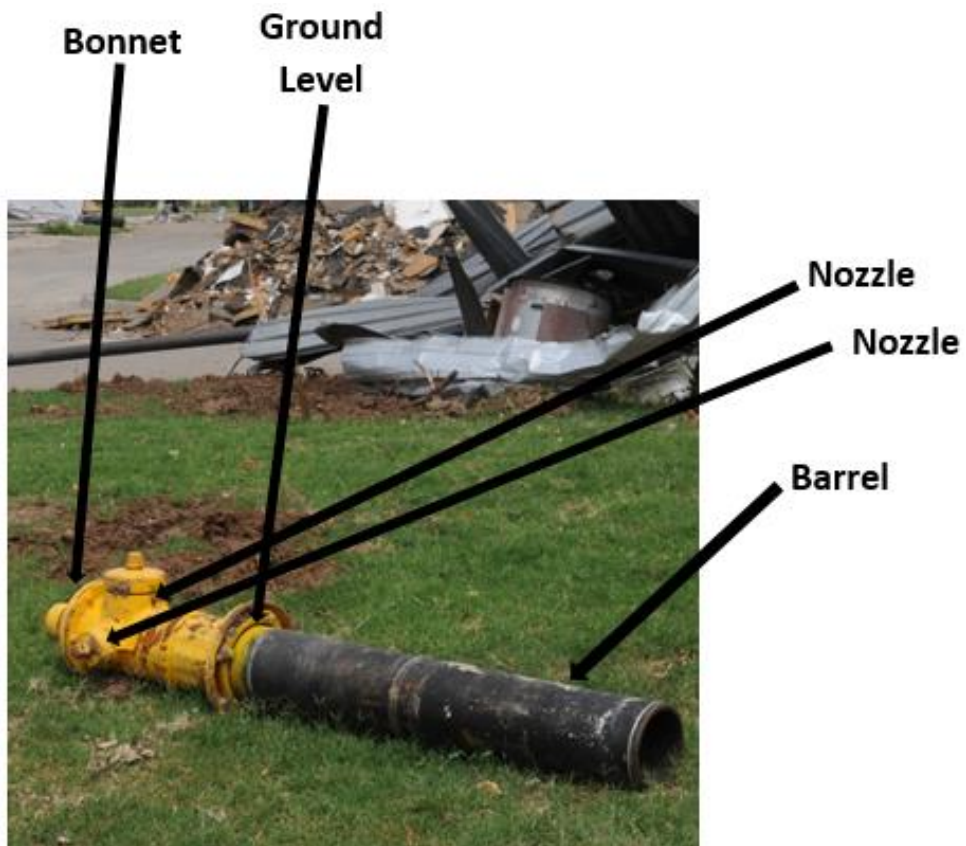
Figure 8.9: The different parts of a fire hydrant 86
