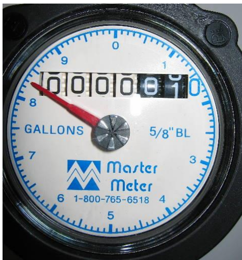
Figure 9.12: A water meter register 100
