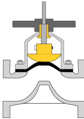
Figure 7.4: A diagram of a rubber lined diaphragm valve 60
