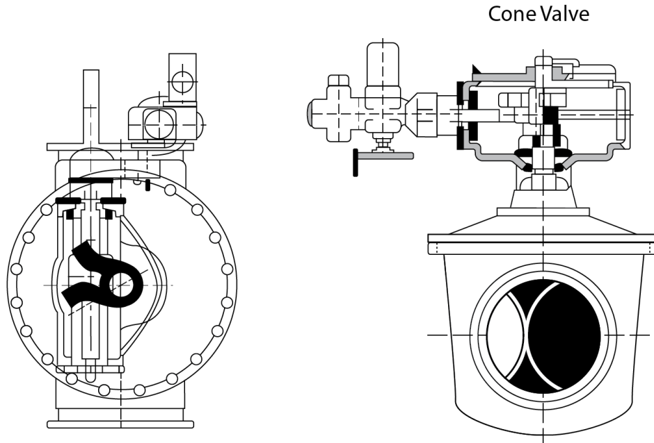
7.11: Cone valve 67
