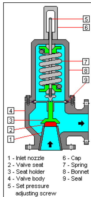
Figure 7.14: The parts of a relief valve 70
