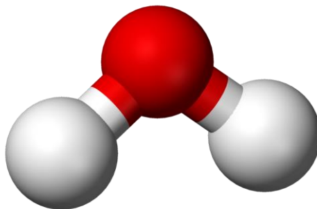
Figure 2.6: Water molecule 15
