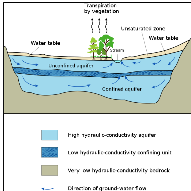
Figure 11.1: An unconfined and confined aquifer 101
