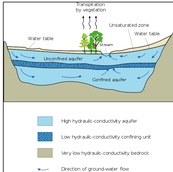
Figure 2.4: Aquifers 13
