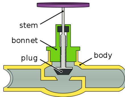
Figure 7.1: A globe valve diagram 57
