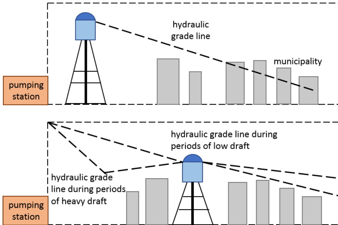
Figure 5.1: Hydraulic grade line diagram 36
